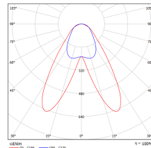
Retail double asymmetric lens (A2)
