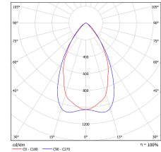
Mid-Wide 60° UGR<19 lens (UGR6)
