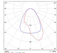
Asymmetric lens (A1)
