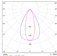
High rack lens for high installations (HR)
