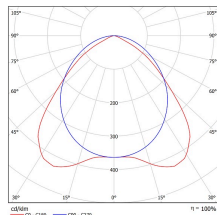
High light output tunnel wide 90° lens (T90)
