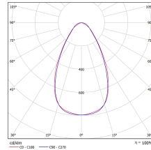
Mid-wide 60° lens (W60)
