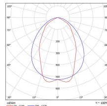
High light output tunnel mid-wide 60° lens (T60)
