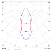
Narrow 30° lens (N30)
