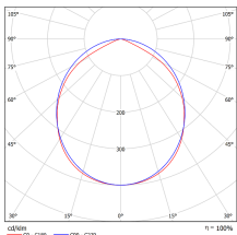
Opal lens (S1)
