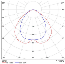
Extra wide 110° lens (W110)
